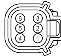
Gasoline Injector Harness Male (M) Female (F)
