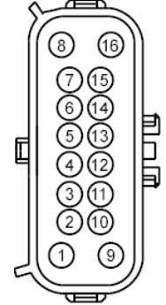
Ford Connector C145 Male (M)
