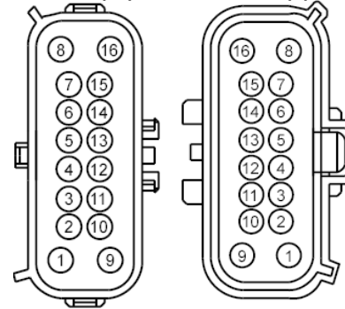
Ford CNG Prep Connector Male (M) Female (F)
