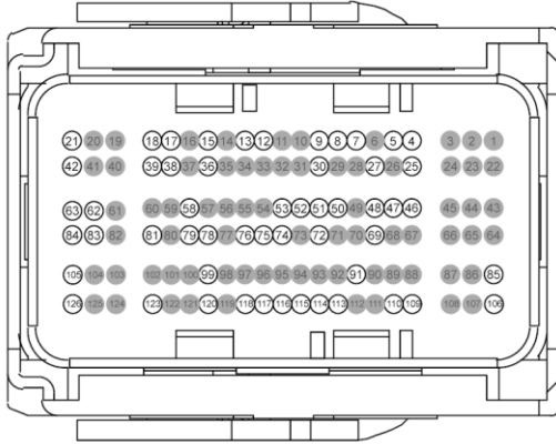
Rear Harness
